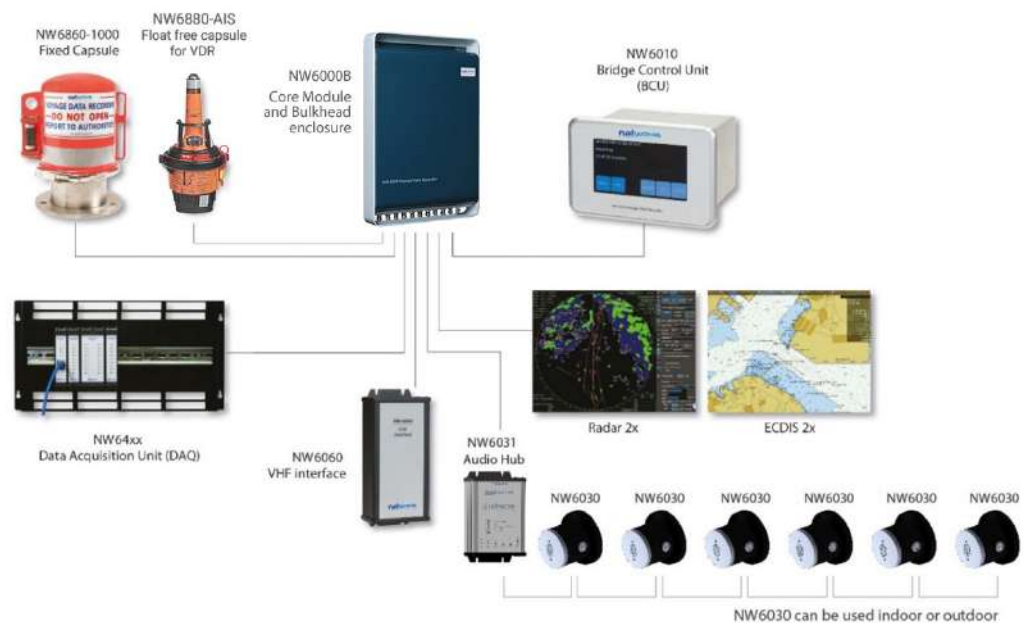
Netwave Voyage Data Recorder Architecture
